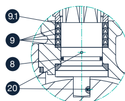
A VIEW
